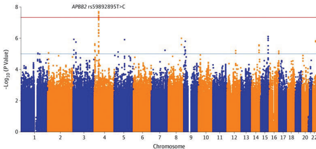
Manhattan plot from GWAS identified new gene on chromosome 4 significantly associated with POAG in African American population
