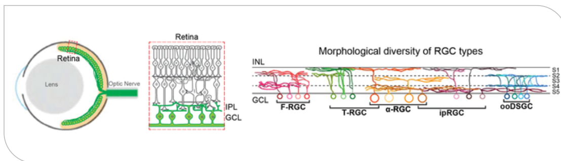
Single cell RNA-seq reveals 45 molecularly distinct RGC types in adult mice
