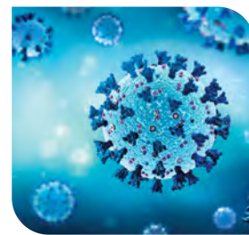
SARS-CoV-2 particles
